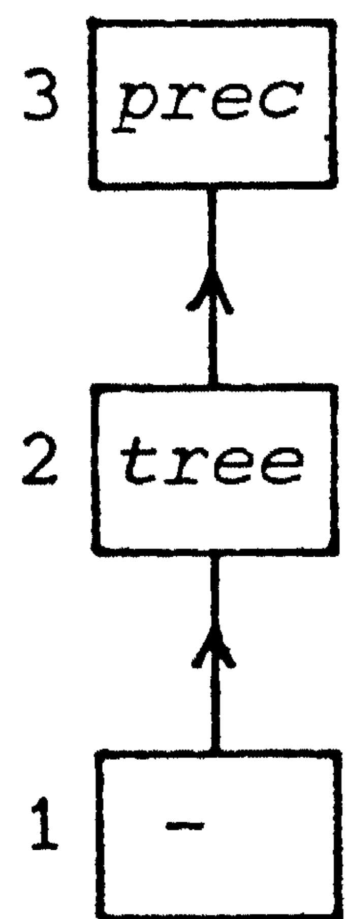
Figure 2 The graph G_2 .
