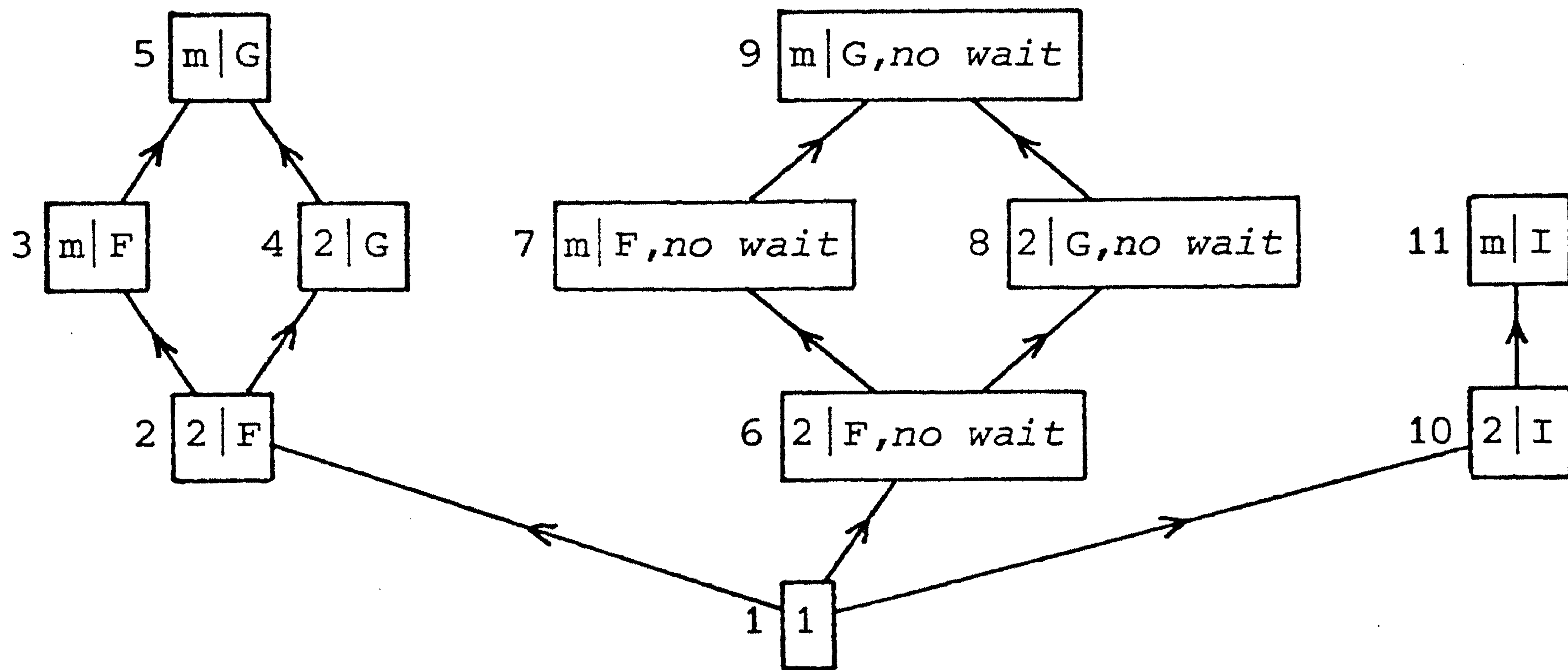
Figure 1 The graph G_1 .
