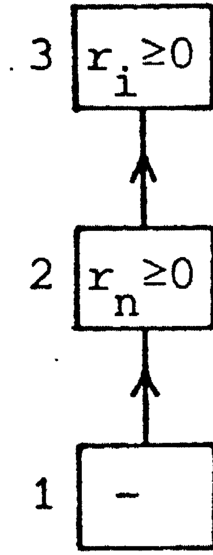
Figure 4 The graph G_4 .
