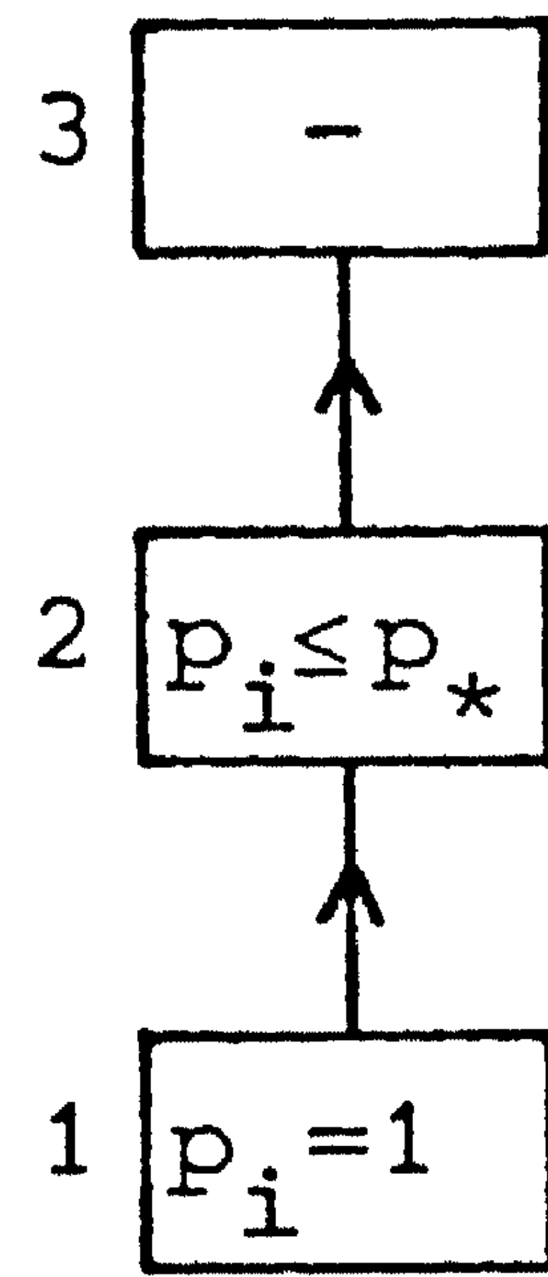
Figure 3 The graph G_3 .
