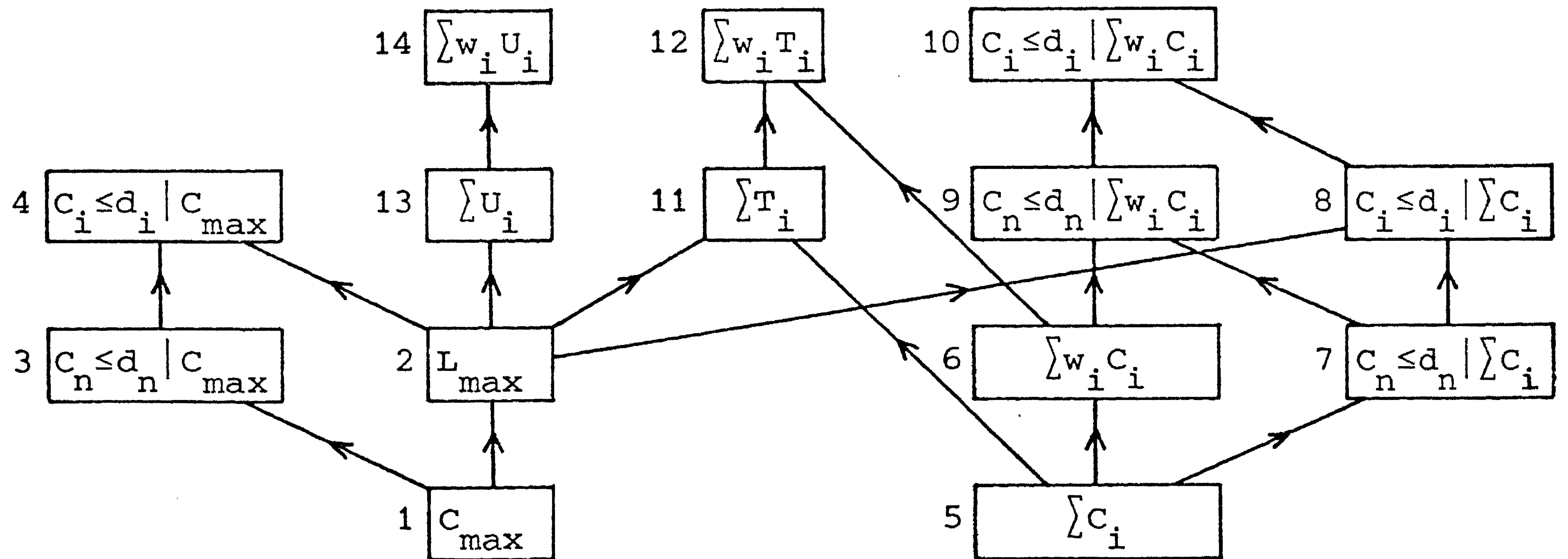
Figure 5 The graph G_5 .
